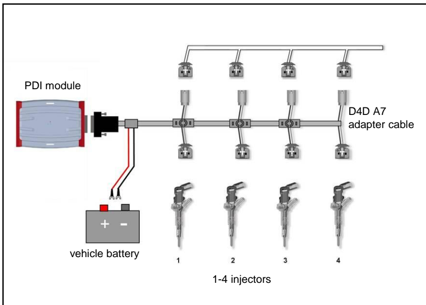
ill.5 installation principle
